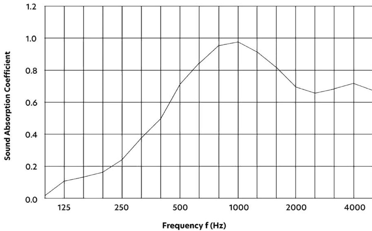
Fig. 01 - The graph illustrates the coefficient of sound absorption at different frequency levels, where human speech is centered between 1,000Hz to 5,000 Hz.
